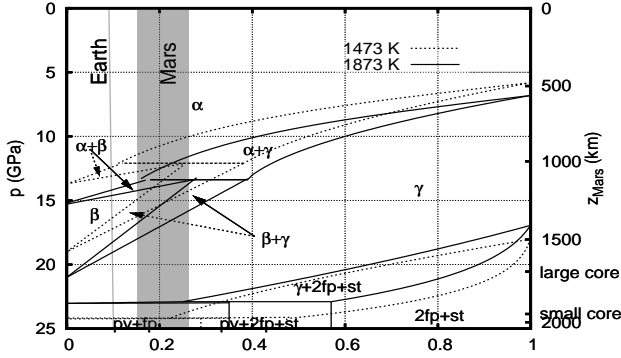
Figure 1: Isothermal phase stability fields of (\text{Mg,Fe})_2\text{SiO}_4 at two different temperatures versus pressure and iron content. The depth scale corresponds to the martian mantle and is approximately valid within the “Mars” interval (shaded) of X_{\text{Fe}} . “Large core” and “small core” refer to bounds on the depth of the core–mantle boundary that include most of the published estimates.
