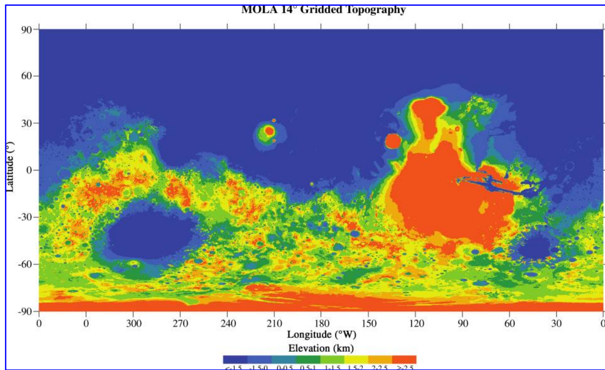
FIG. 9.2. Mercator projection of 1/4 gridded Mars Orbiter Laser Altimeter (MOLA) topography of Mars from 90°S to 90°N latitude, showing the areas below +1 km elevation in blue and dark green. Elevation is relative to the MOLA datum (Smith et al. , 2001). This map uses an areocentric coordinate convention with west longitude positive. Image Credit: NASA/JPL-Caltech/GSFC.
